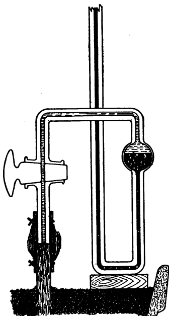
FIG. 33.—Apparatus for the demonstration of Root Pressure; \times \frac{1}{2} .
